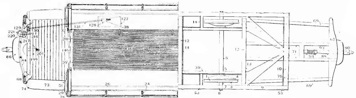
Fig. 5655. Half Plan of Car Floor and Half Plan of Underframe.
